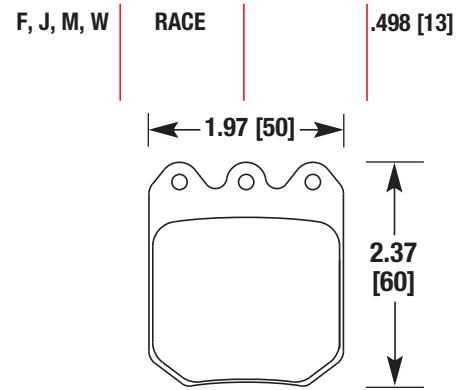
WILWOOD 6812
