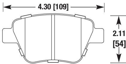
VOLKSWAGEN, AUDI (REAR)
