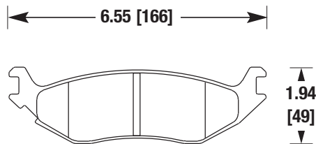
DODGE TRUCK (REAR)
