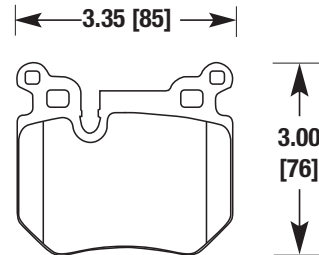
BMW 135i (REAR)
