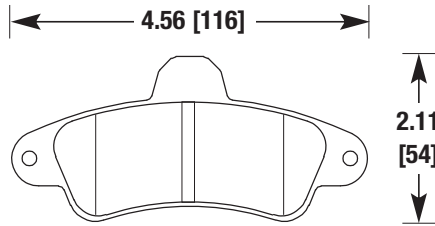
FORD MERCURY (REAR)
