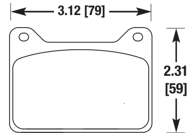
WILWOOD 7912
