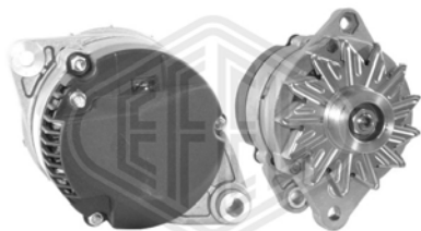
AA125R - 14V - 65A - pulley PolyV-5
