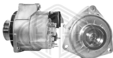
NL1 - 28V - 100A - pulley PolyV-9
