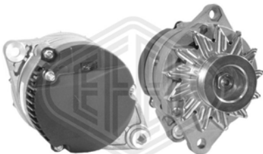
AA125R - 14V - 65A - pulley PolyV-5
