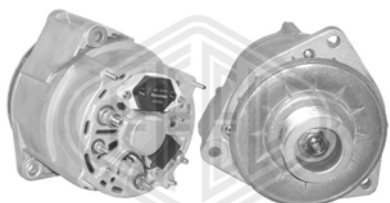
NL1 - 28V - 100A - pulley PolyV-8
