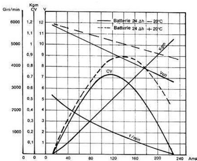
Performance curve of dynamo
