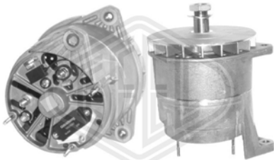
T1 - 28V - 185A - (Fan wheel)
