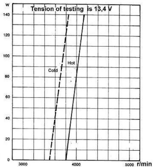
Performance curve of starter
