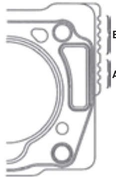
Joint métallique multifeuille Multi-layer steel gasket (ELRING)
