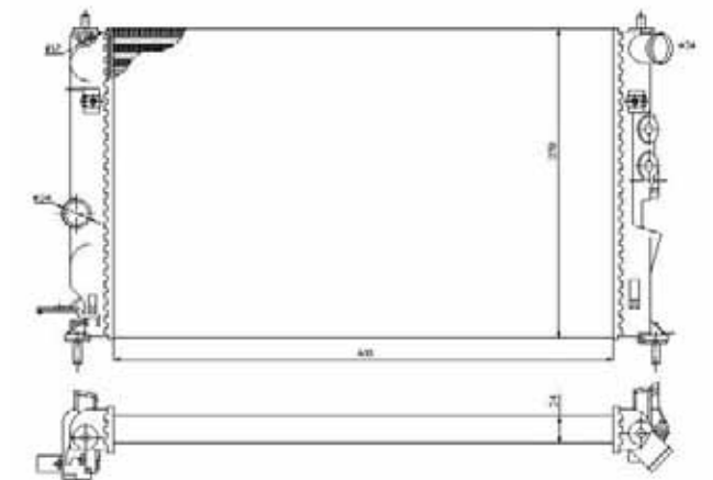
TYC 725-0027-R
