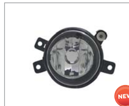
Fog Lamp Unit 19-12103-01-9 RH 19-12104-01-9 LH 63172993526 63172993525 (E13) For standard bumper, not used with AFS
